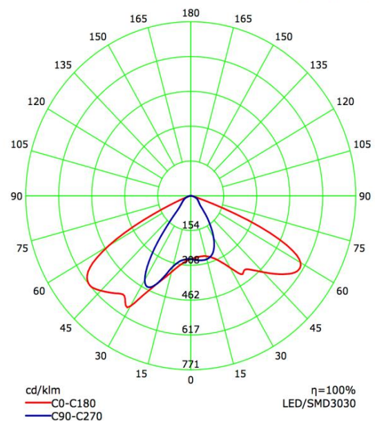
Luminous Intensity Distribution Curve(cd/klm)
